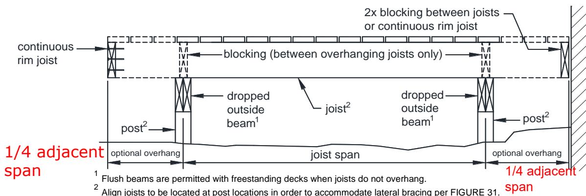
FIGURE 9: JOISTS WITH FREESTANDING DECKS
