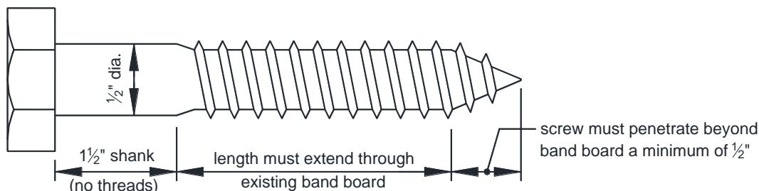
FIGURE 27: LAG SCREW
